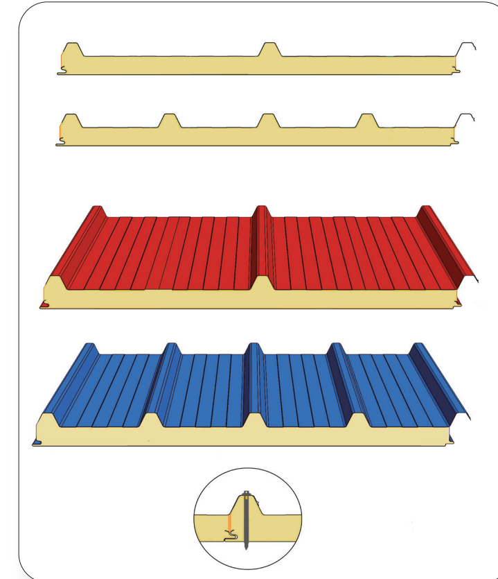
Roof Panel
